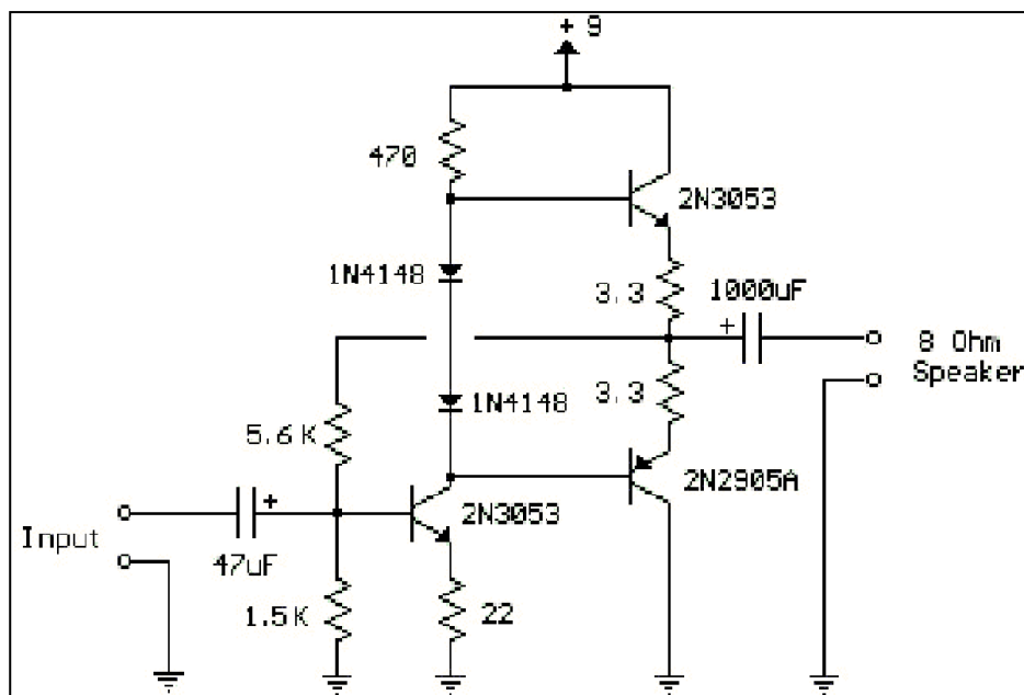
Transistor Audio Amp (50 mW)
